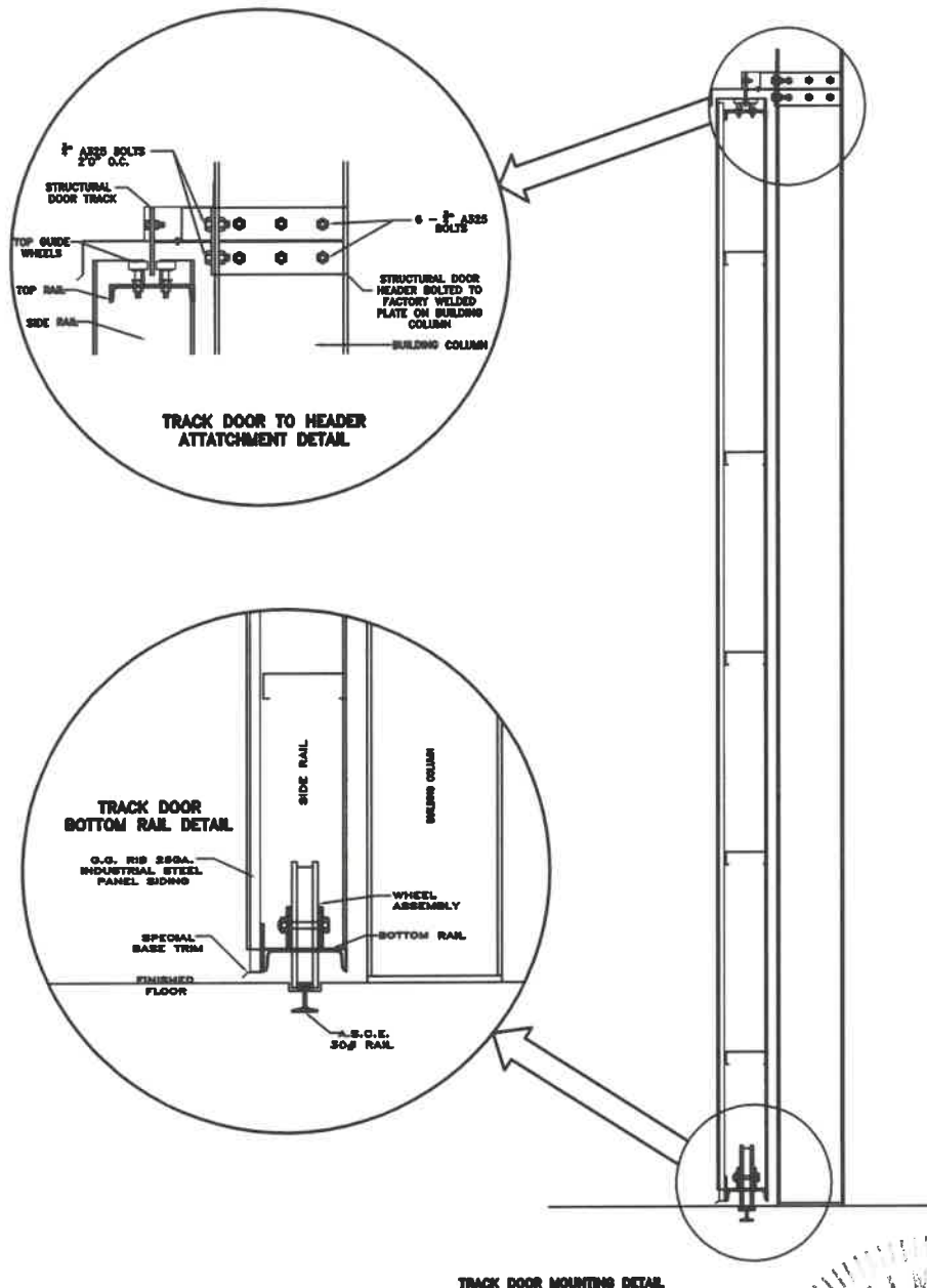
TRACK DOOR MOUNTING DETAIL
