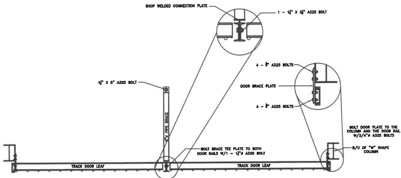
BOTTOM MOUNT TRACK DOOR HIGH WIND BRACE ATTACHMENT DETAIL
