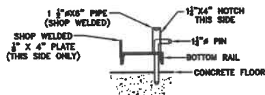
BOTTOM MOUNT TRACK DOOR ANCHOR DETAIL
