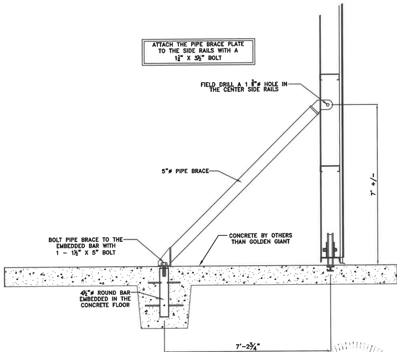
TRACK DOOR BRACE DETAIL
